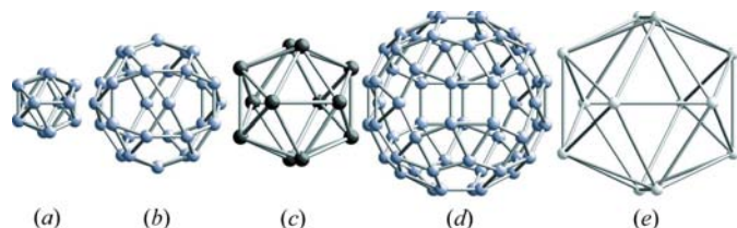
Figure 4 Shells of the double-Mackay cluster (Sugiyama et al. , 1998) building the approximant c P138- \alpha -Al–Mn–Si. The shells (a)–(e) are centred at the origin of the unit cell and shells (a)–(c) in the body centre as well. Shells (a)–(c) form the 54 atom Mackay cluster. (a) Al/Si icosahedron. If the icosahedral symmetry is broken by this innermost shell, the pseudo-Mackay cluster is obtained (Boudard et al. , 1992). (b) Al icosidodecahedron. Its pentagons are capped by Mn atoms forming an icosahedron with diameter similar to the icosidodecahedron (c). (d) Complex Al shell. (e) Icosahedral Al/Si shell.
