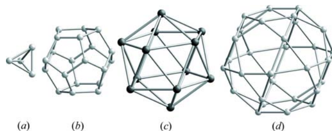
Figure 6 Shells of the 66 atom Tsai cluster building c I168-Cd 6 Yb (Takakura, Shiono et al. , 2001). All shells are centred at the origin. (a) Orientationally disordered Cd tetrahedron. (b) Cd pentagondodecahedron. The pentagons are capped by Yb forming an icosahedron (c). (d) Cd icosidodecahedron.
