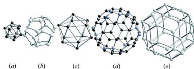
Figure 5 Shells of the 104 atom Samson cluster building the approximant c I160- R -Al 3 CuLi 3 (Audier et al. , 1988). All shells are centred at the origin. Shells (a)–(c) form the 44 atom Bergman cluster. (a) Al/Cu icosahedron. (b) Li pentagondodecahedron. Its pentagons are capped by Al/Cu atoms forming an icosahedron with diameter similar to the dodecahedron (c). These two shells together form a triacontahedron. (d) Truncated icosahedron of Al/Cu atoms. (e) Li triacontahedron with Li atoms capping the hexagonal faces of the truncated icosahedron.
